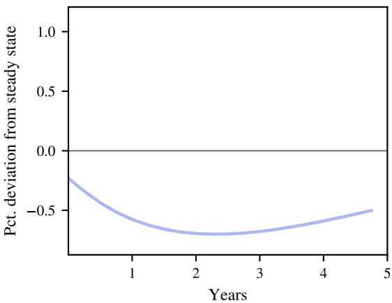
Non-tradable price
